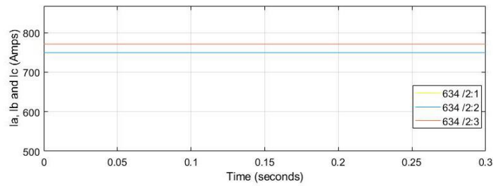
Fig. 9: Bus 634 three-phase currents at steady-state.
