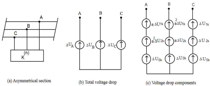
Fig. 2: General case of transverse asymmetry.
